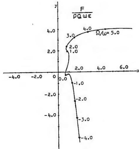
Fig. 5 Vector diagram of radial forces on whirling impeller ( N=6 , \beta=30^\circ , r_1/r_2=0.5 , \Gamma_p=0 , \psi=0.433 )
